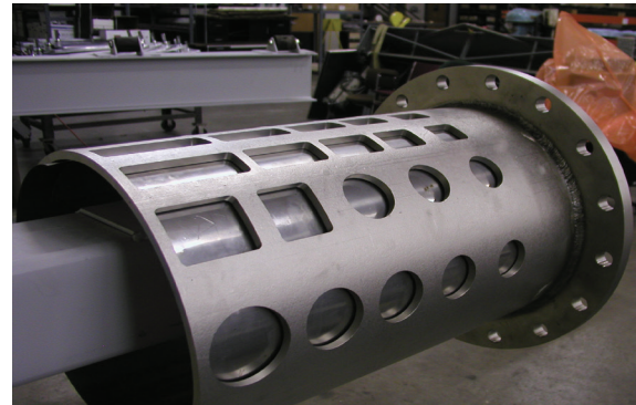
BWR Strainer, Sure-Flow
